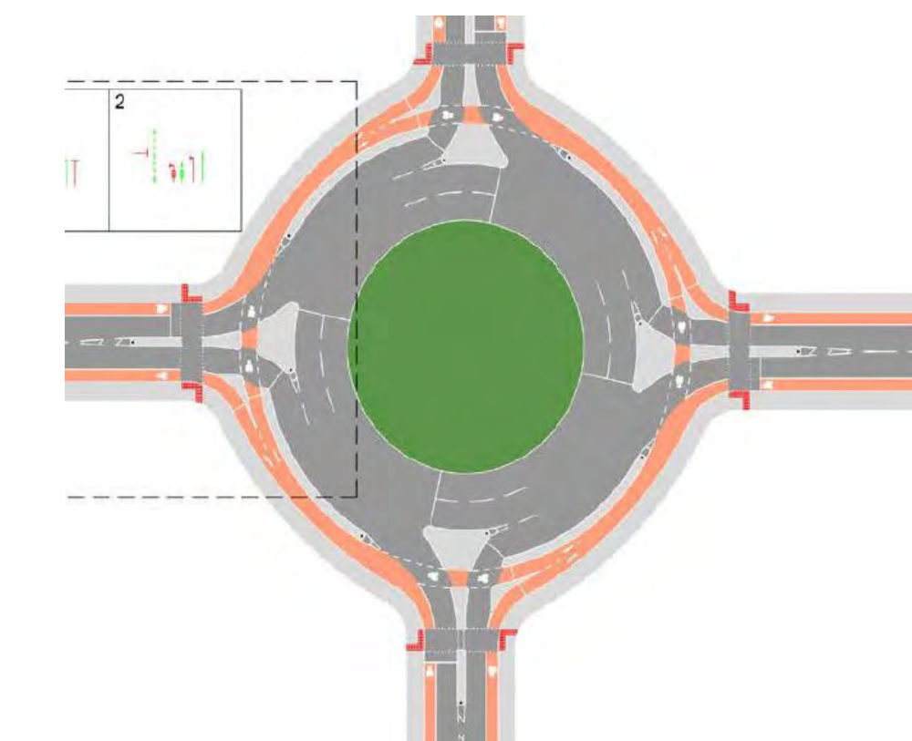
Figure 10.39: Carriageway-level cycle track used with ‘hold the left’ traffic staging
